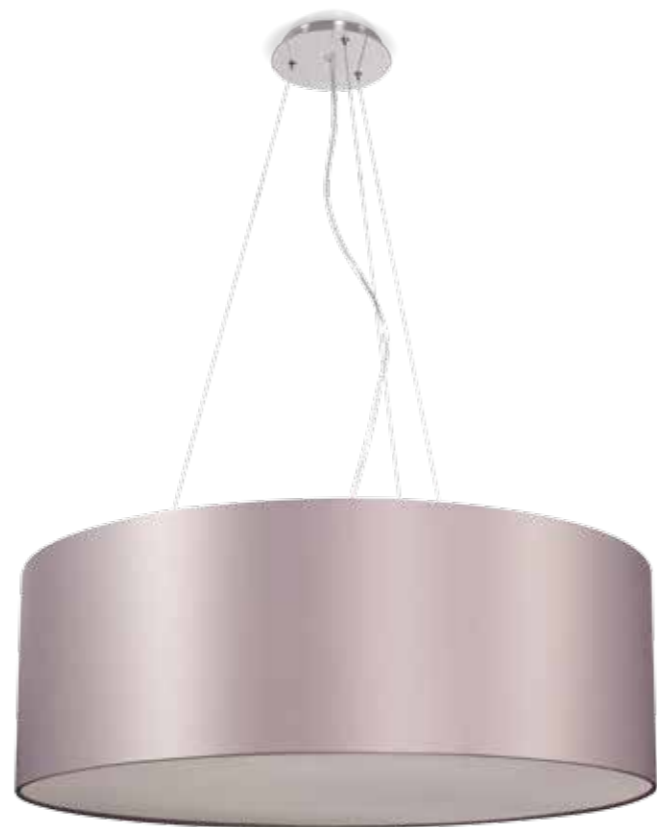
148/S CROMO | Ø 16 cm | 120 cm | 3 x E27 / 60W COR 509 | 80x80x30 cm
